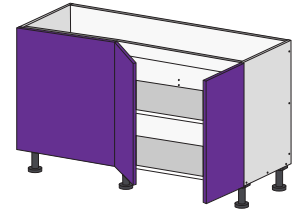
Base Return Pair Doors
